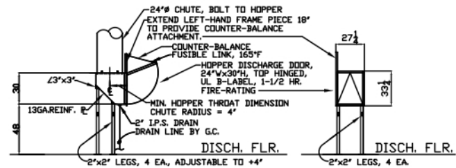
CHUTE DISCHARGE DRAWING CHUTE DISCHARGE DRAWING (24" CHUTE SHOWN) (24" CHUTE SHOWN) (SIDE VIEW) (FRONT VIEW)
