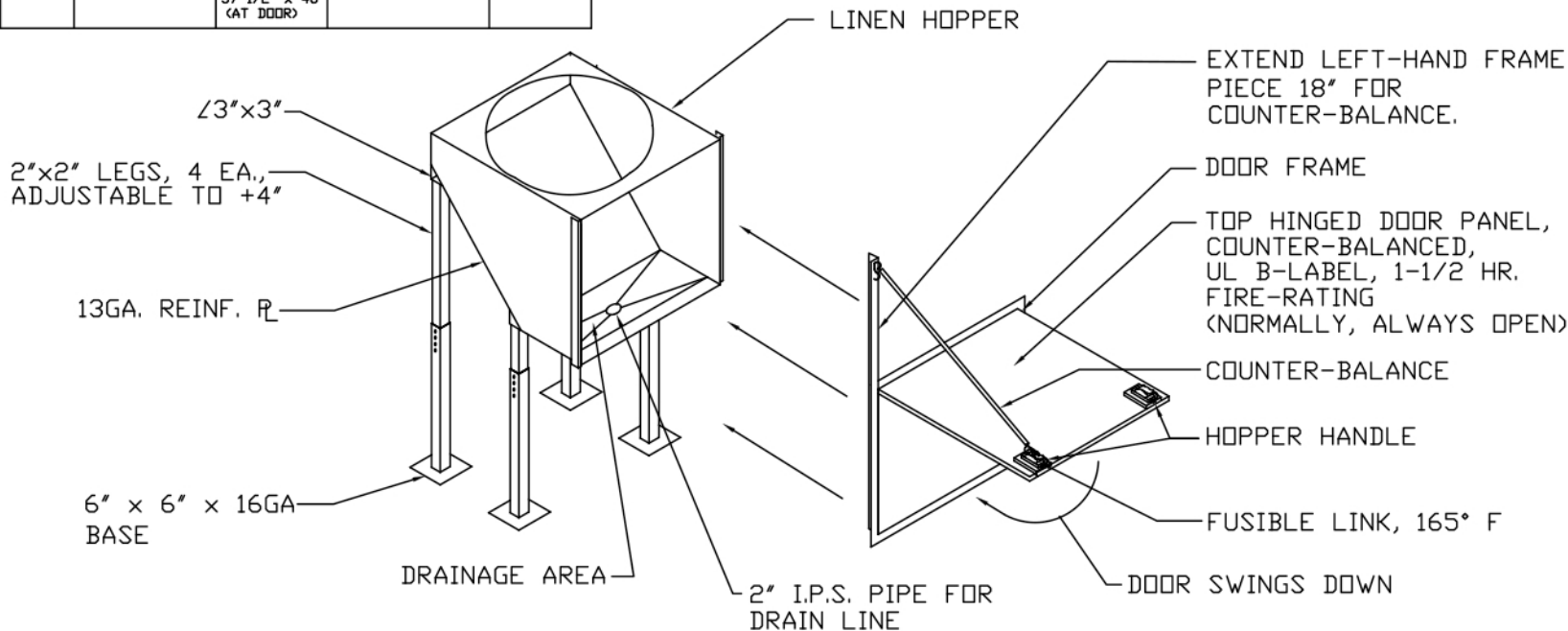
CHUTE DISCHARGE DRAWING CHUTE DISCHARGE DRAWING (24" CHUTE SHOWN) (24" CHUTE SHOWN) (SIDE VIEW) (FRONT VIEW)
