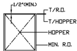
HOPPER & R.O. (FRONT VIEW)
